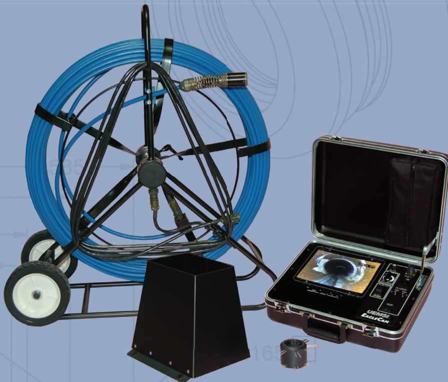
The EagleCam PCU is shown with the reel w/200' of video push cable and the CM-1 color camera head.
